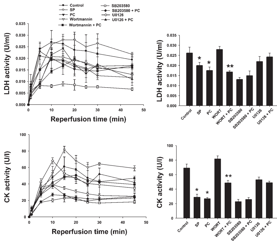
Fig. 2. PC attenuates I/R-induced lactate dehydrogenase (LDH) and creatine kinase (CK) release in coronary effluent from hearts subjected to 30 min of global ischemia followed by 45 min of reperfusion. LDH and CK data are shown as a function of reperfusion time (left) and at 15 min of reperfusion (right). See Fig. 1 legend for treatment protocol. Values are means \pm SD from 6 independent experiments. * P < 0.001 vs. control. ** P < 0.001 vs. wortmannin. PC and SP significantly attenuated LDH and CK release.
