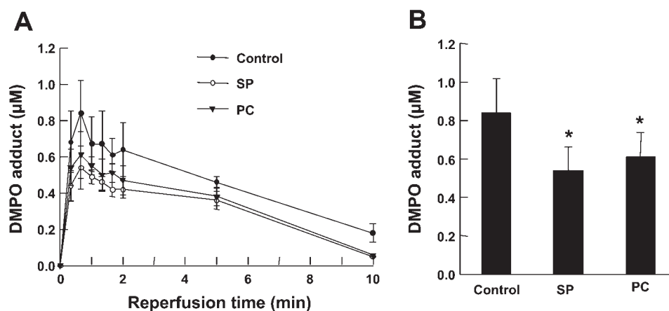
Fig. 4. PC attenuates generation of free radicals during reperfusion. A: time course of 5,5-dimethyl-1-pyrroline- N -oxide (DMPO) adduct. B: DMPO adduct at 1 min of reperfusion. Free radical generation was measured using the spin-trap DMPO with and without PC or SP in hearts subjected to 30 min of ischemia followed by 45 min of reperfusion. DMPO (40 mM final concentration) was infused through a sidearm during reperfusion, coronary effluent was collected at 0.5–10 min, and DMPO adduct formation was measured by electron paramagnetic resonance spectroscopy. Values are means \pm SD from 3 independent experiments. * P < 0.05 vs. control. PC and SP significantly attenuated I/R-induced free radical formation.
